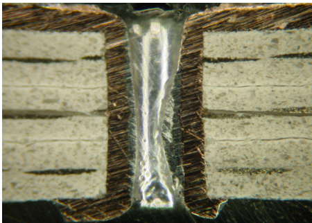
Cross-section of RF-35A2 construction
